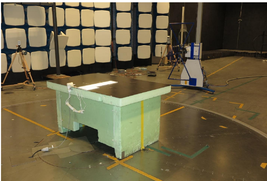
Test set up radiated emission 30 – 1000 MHz, EUT-sample A
