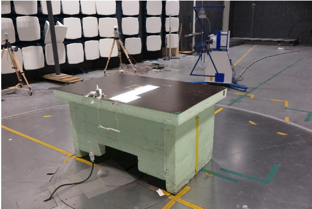
Test set up radiated emission 30 – 1000 MHz, EUT-sample B
