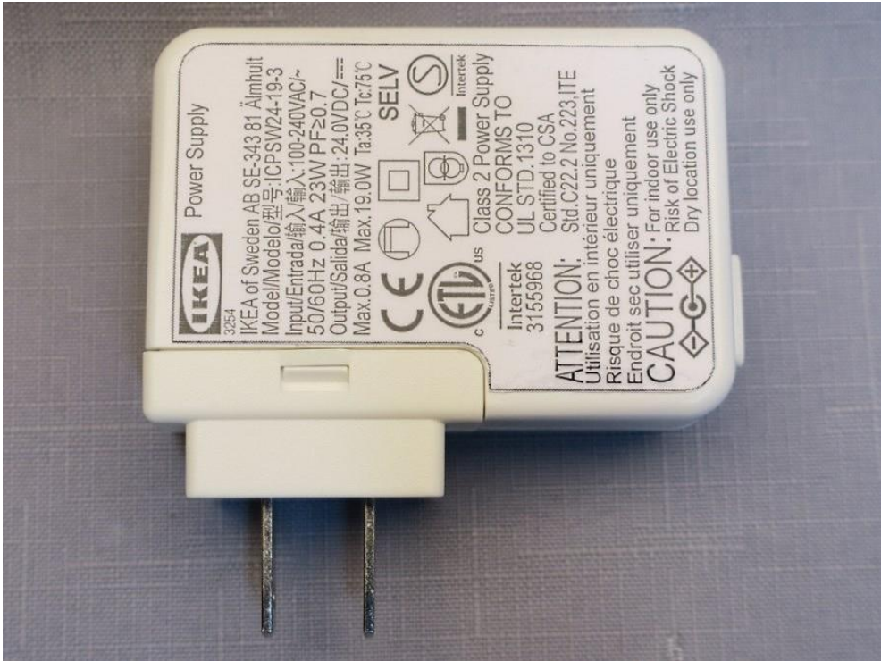
Photo 1 - External view (with mounted optional mains plug)
