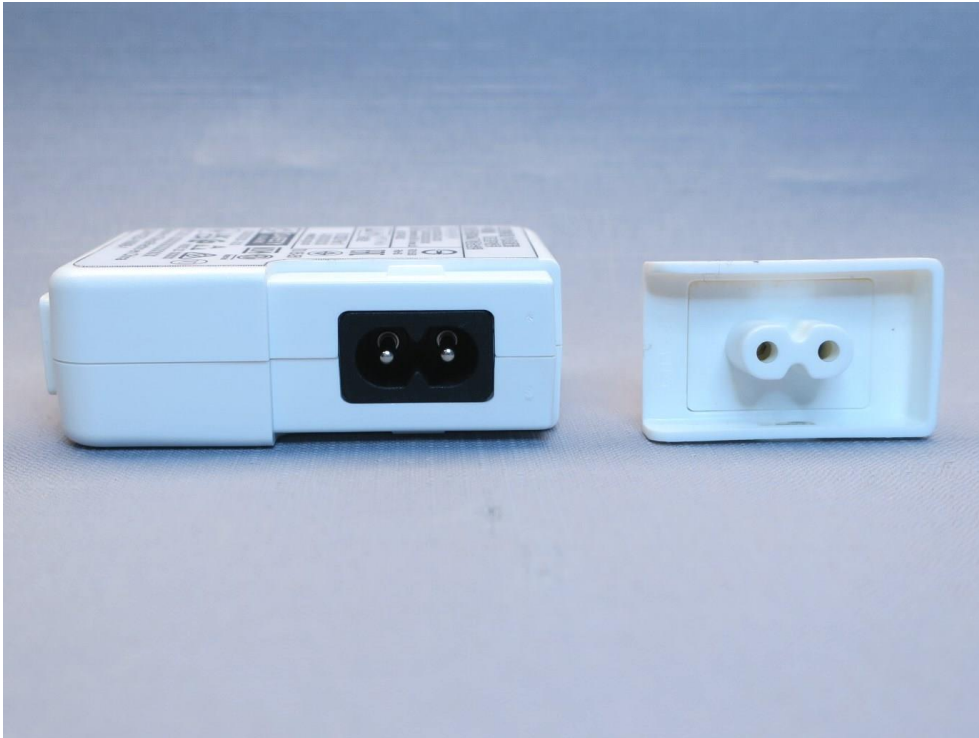
Photo 3 - View of the plug part removed (without the optional mains plug)
