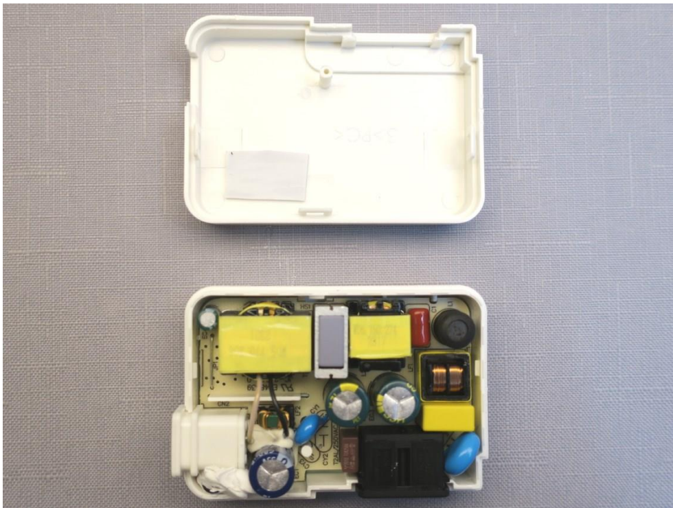
Photo 8 - Internal view of ICPSW24-19-3
