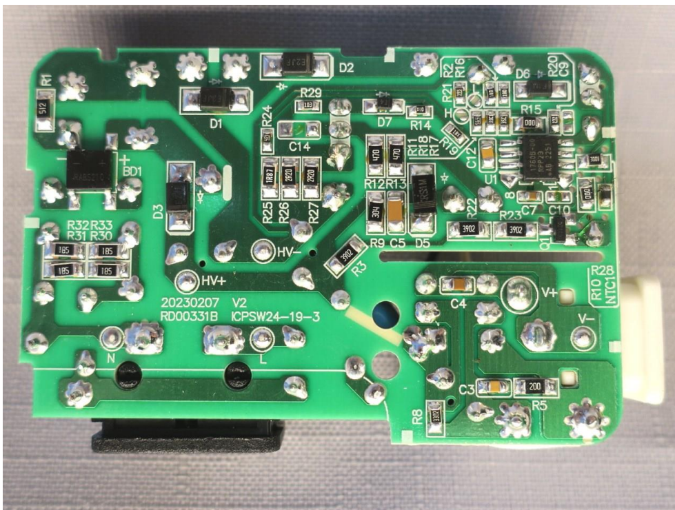
Photo 10 - View of PWB rear side, of ICPSW24-19-3
