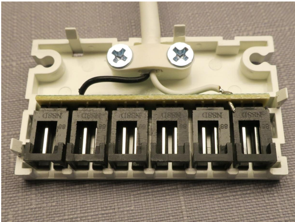
Photo 14 - Internal view of connector hub for the Optional output cord-set
