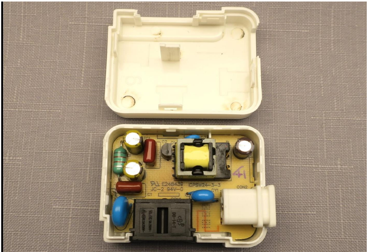
Photo 6 - Internal view of ICPSW24-3-3
