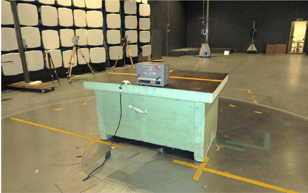
Test set up radiated emission 30 MHz – 1 GHz
