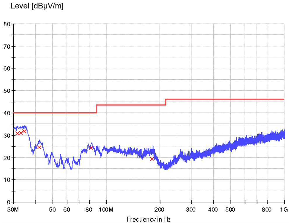
Figure 4: Spectral Diagrams, Radiated Emission, 30 MHz – 1000 MHz, Vertical polarization
