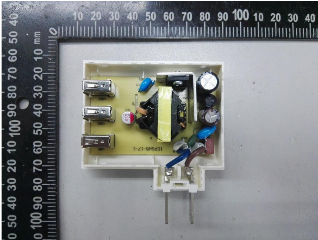
Photo 2 - Internal view
