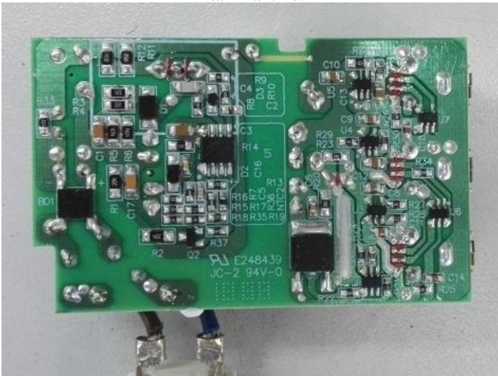
Photo 4 - Internal view
