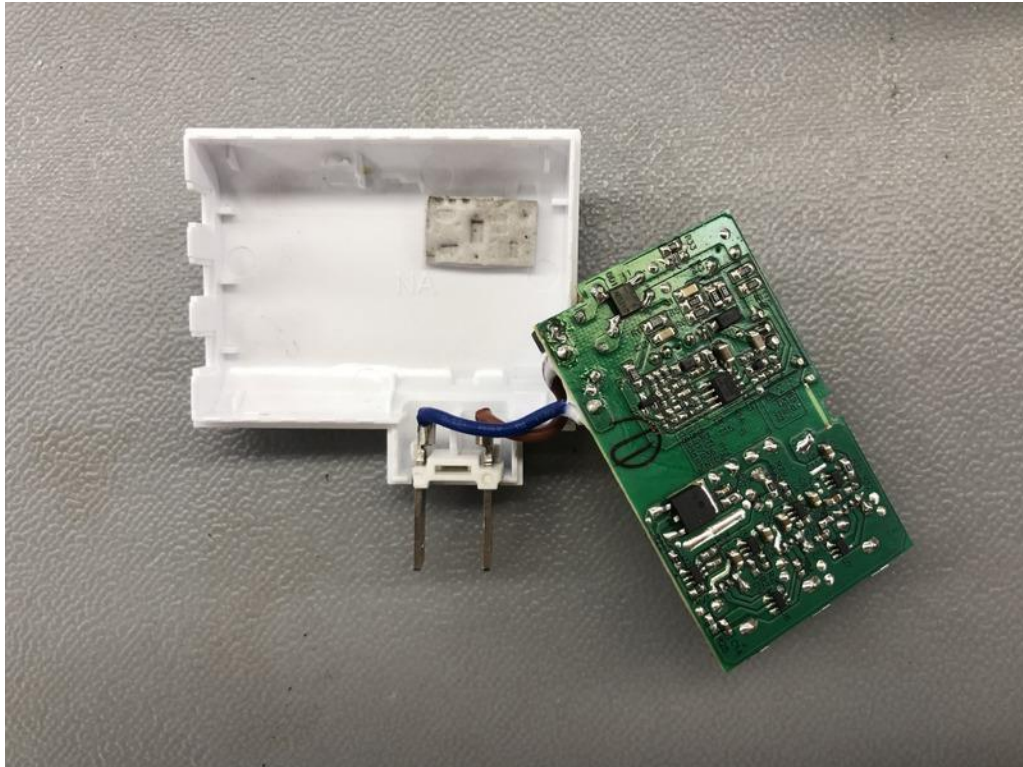
Photo 4 - Internal view
