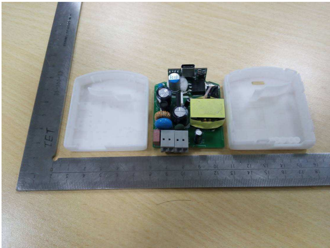
Picture 4 – Internal view (with perpendicular output connector)
