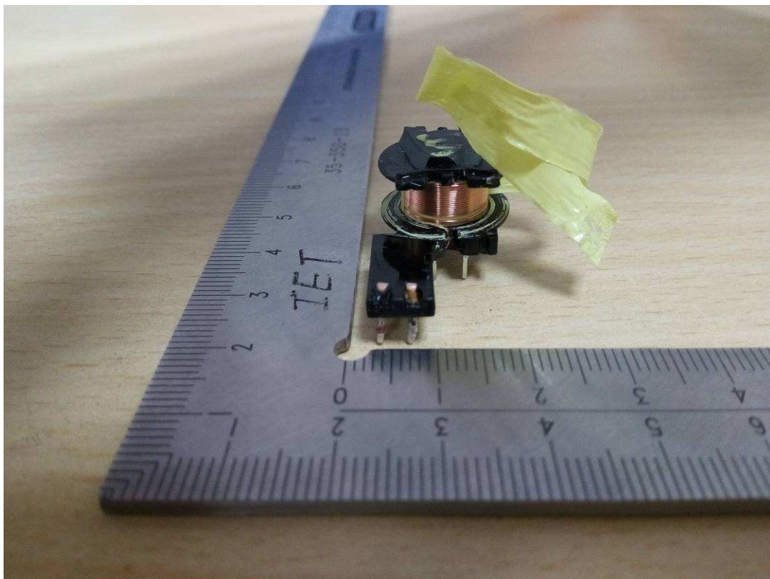
Picture 16 – Transformer view
