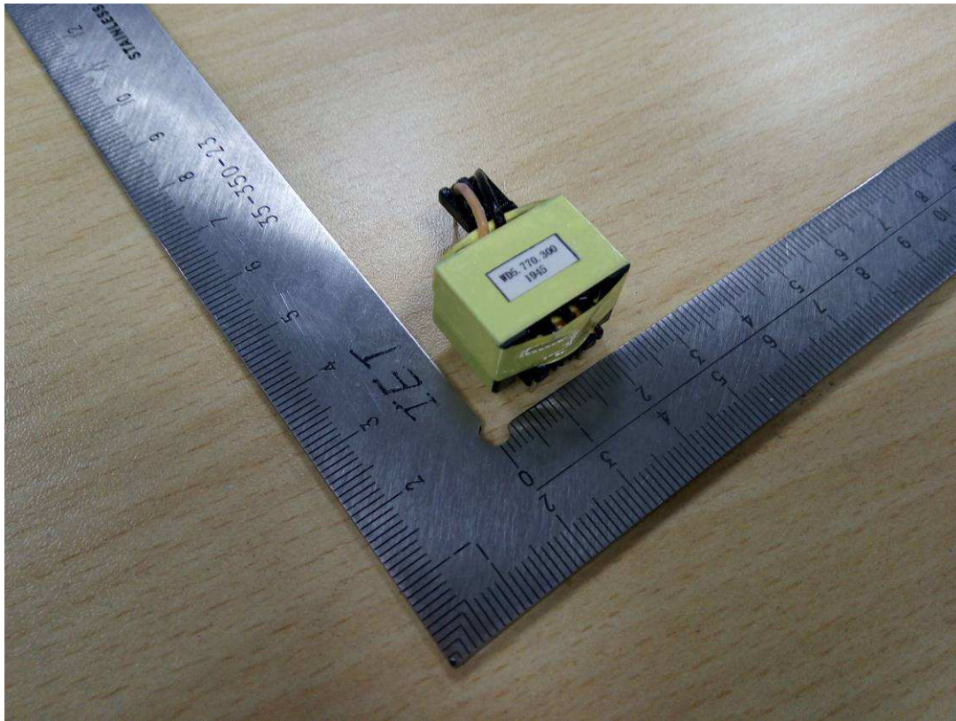
Picture 5 – Transformer view
