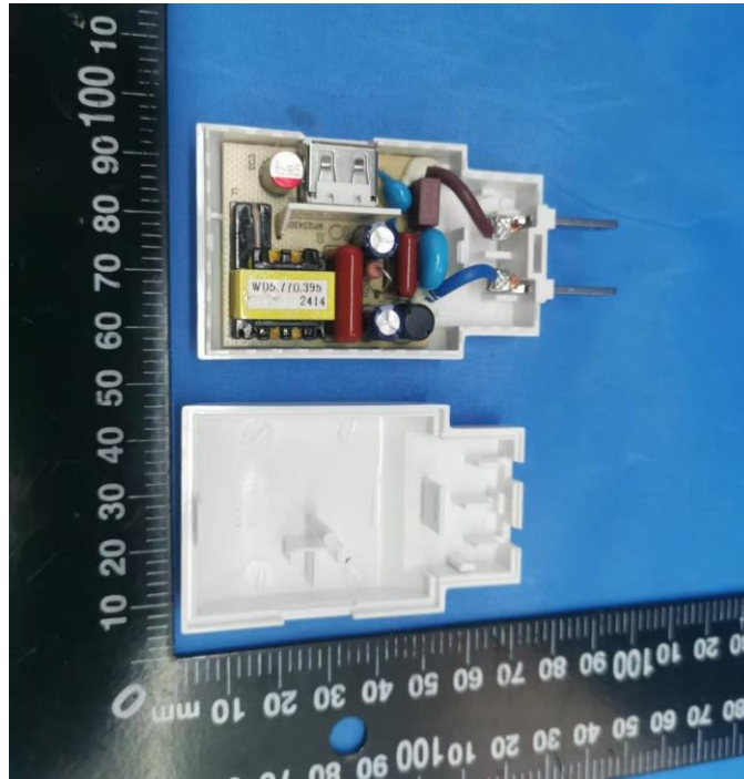
Photo 2 - Internal view
