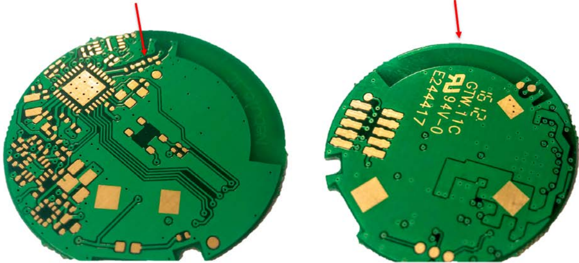
Antenna matching area
