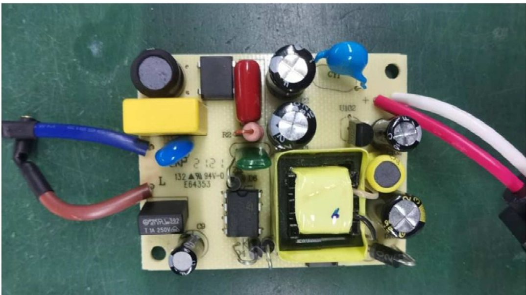
View of PCB
