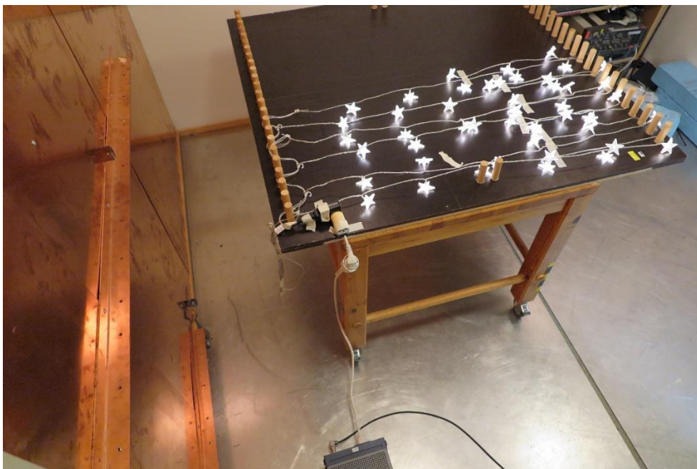
Test setup for conducted emission 150 kHz – 30 MHz
