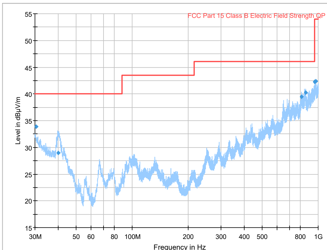
Diagram, Peak overview sweep, 30 – 1000 MHz at 3 m.
