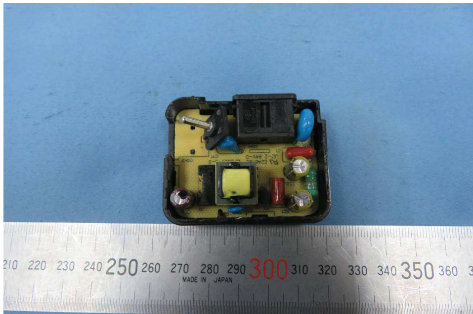
adaptor ICPSW24-3-3 PCB view
