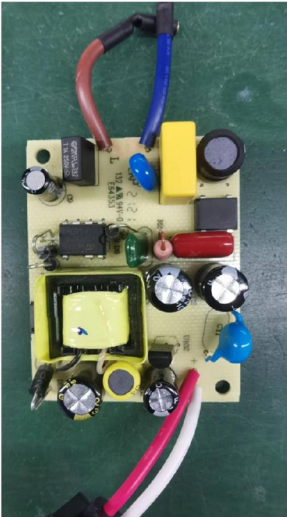
J2201 GOKVÄLLÅ – LED with & decoration photo :
