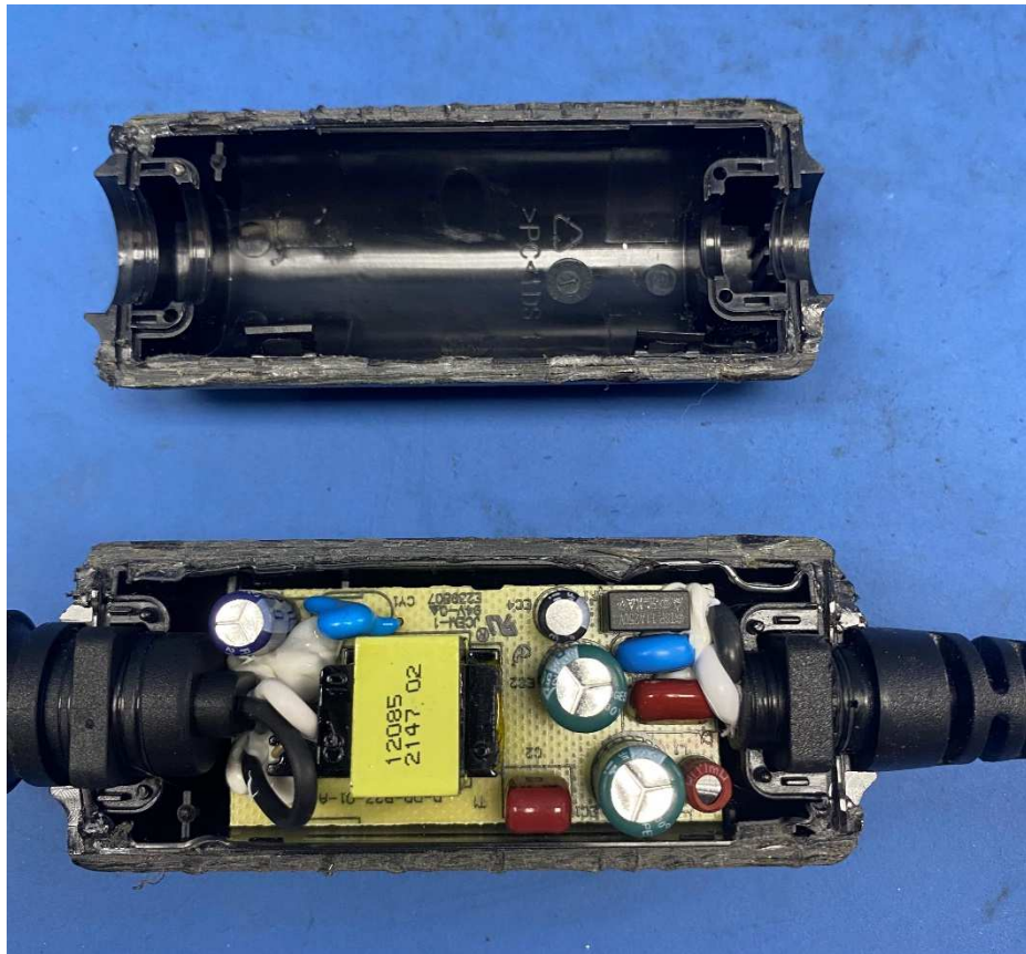
Power unit internal view
