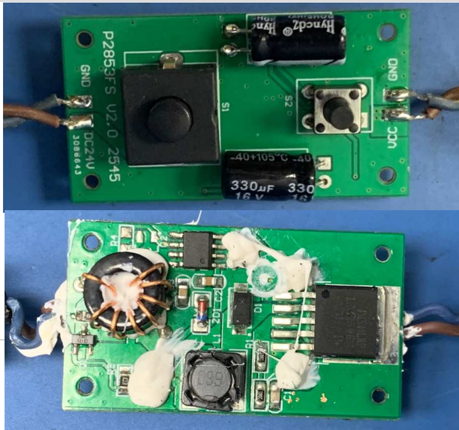
Controller PCB view
