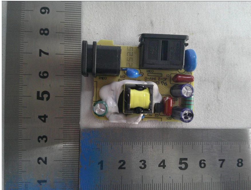
PCB of LED power supply
