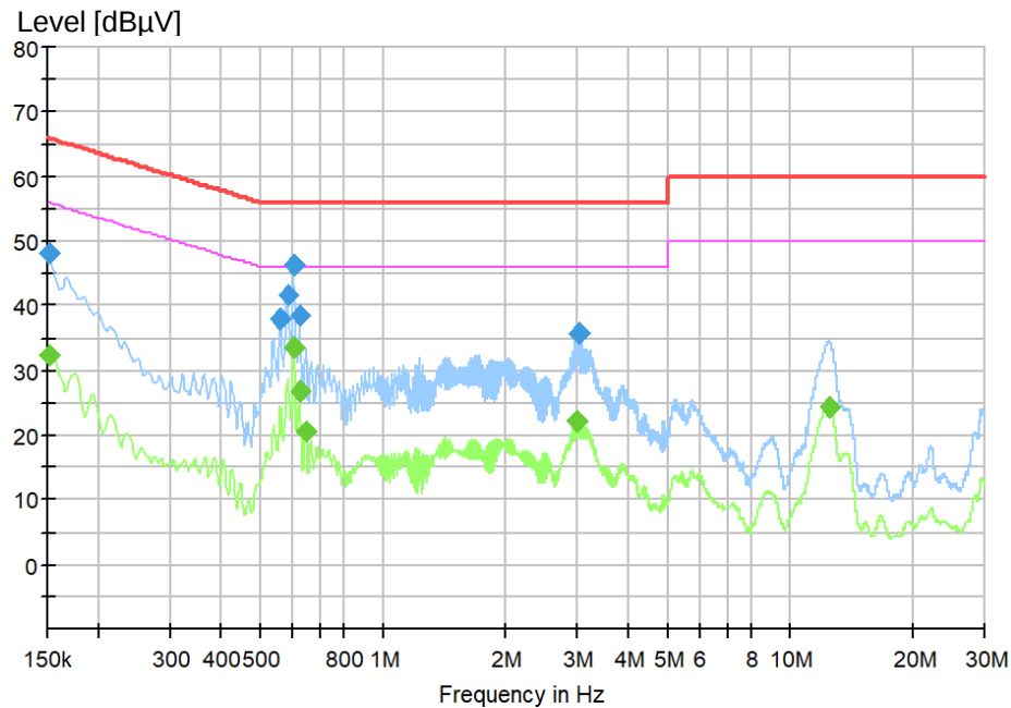
Figure 1: Spectral Diagrams, Conducted Emission, 150 kHz – 30 MHz, L
