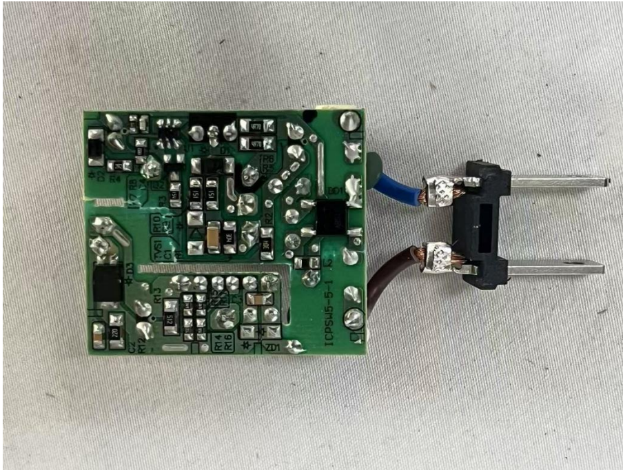
Open View for Power supply
