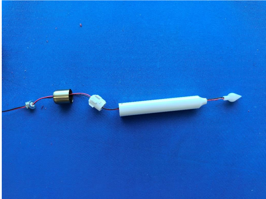
Open View for LED light
