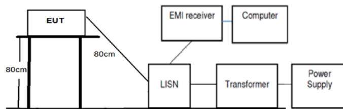
(Conducted emission)
