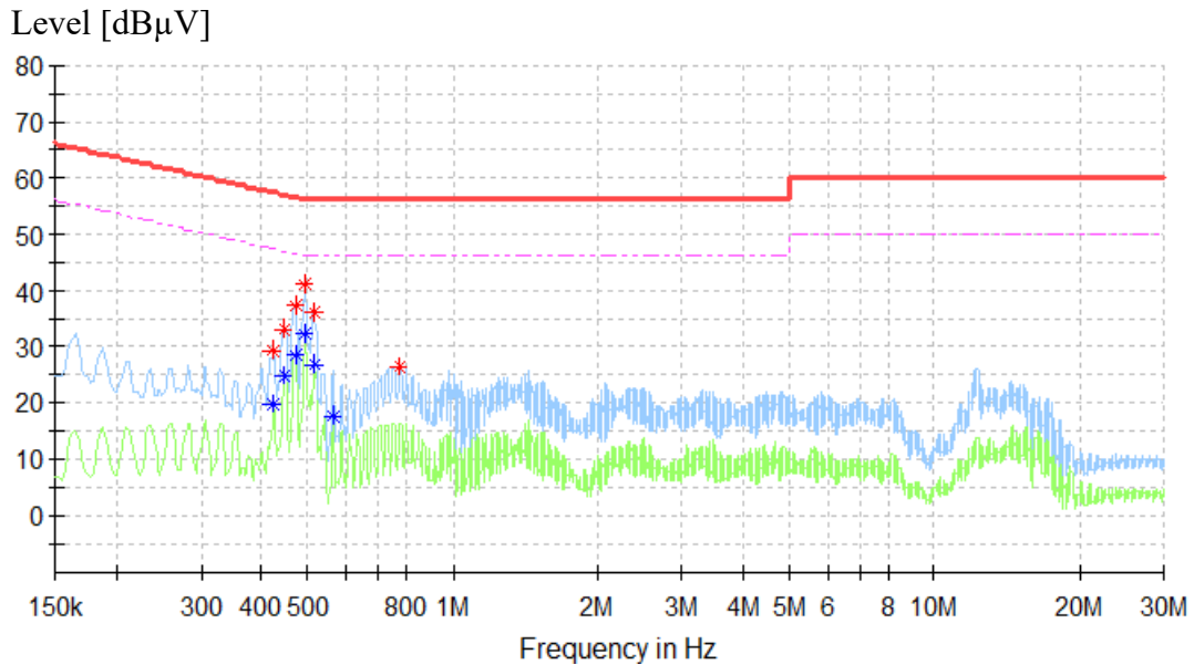
Figure 1: Spectral Diagrams, Conducted Emission, 150 kHz – 30 MHz, Line L
