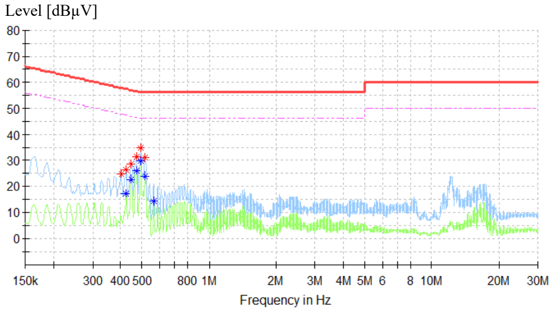
Figure 2: Spectral Diagrams, Conducted Emission, 150 kHz – 30 MHz, Line N
