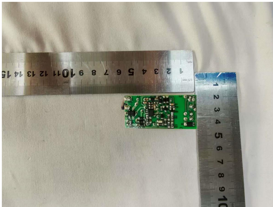
The PCB of LED power supply
