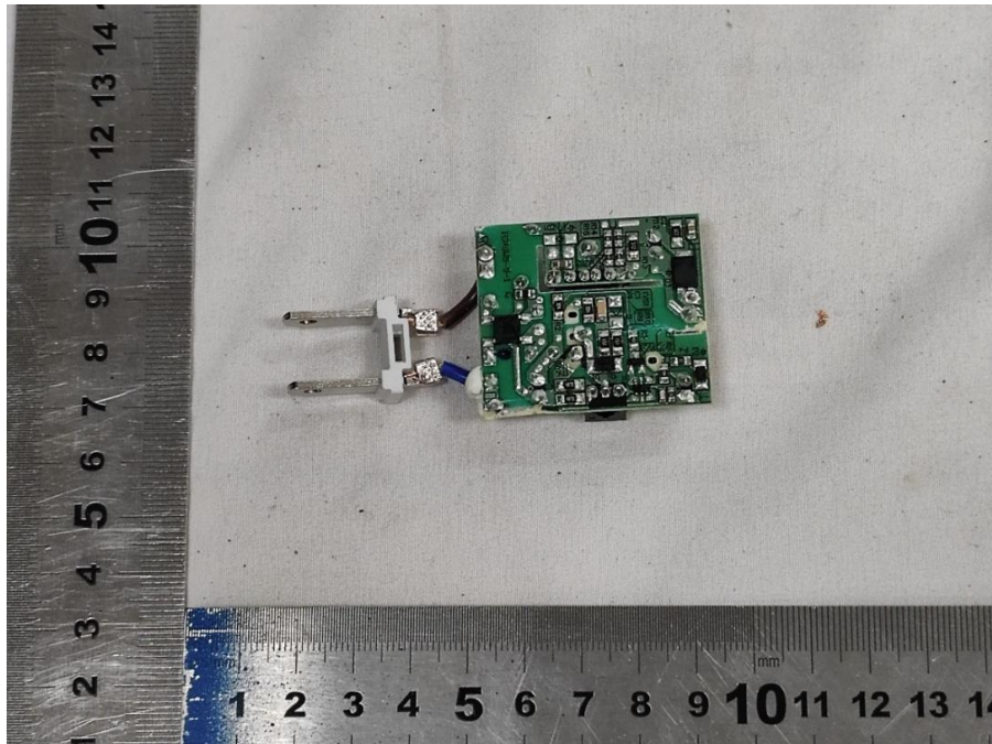
PCB of power supply
