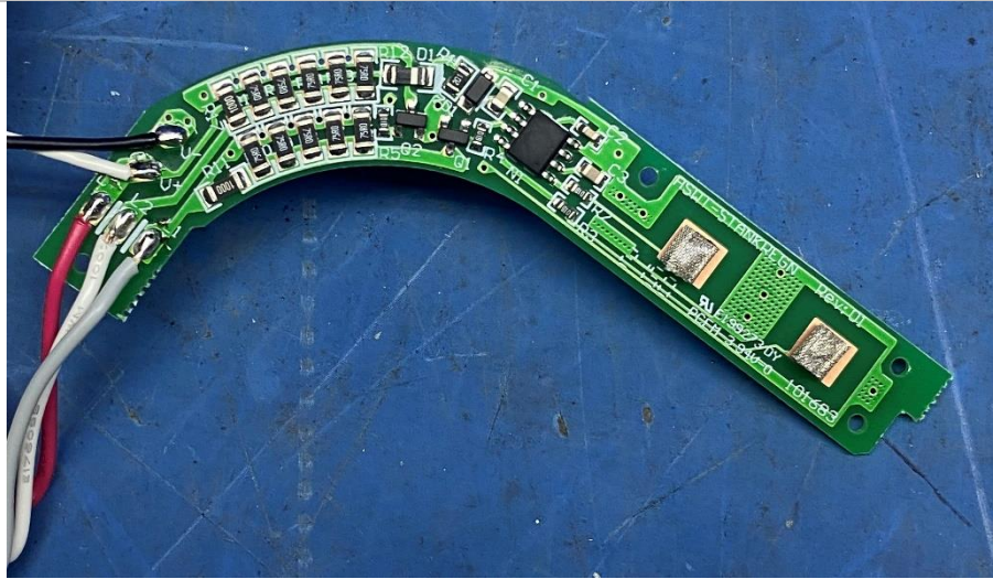
PCB View
