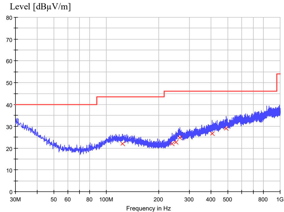
Figure 7: Spectral diagrams, radiated emission, 30 MHz – 1000 MHz, mode 2, horizontal polarization
