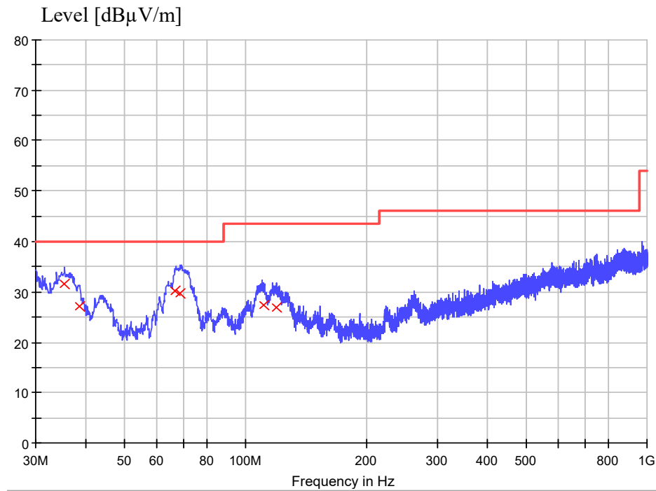
Figure 6: Spectral diagrams, radiated emission, 30 MHz – 1000 MHz, mode 1, vertical polarization
