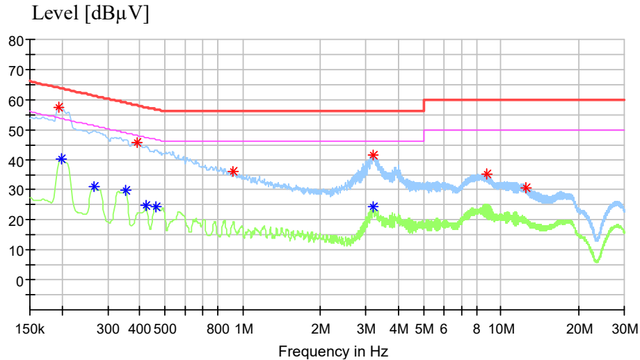
Figure 1: Spectral Diagrams, Conducted Emission, 150 kHz – 30 MHz, mode 1, L line
