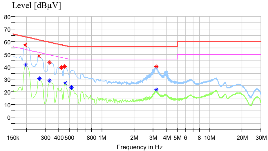
Figure 2: Spectral Diagrams, Conducted Emission, 150 kHz – 30 MHz, mode 1, N line
