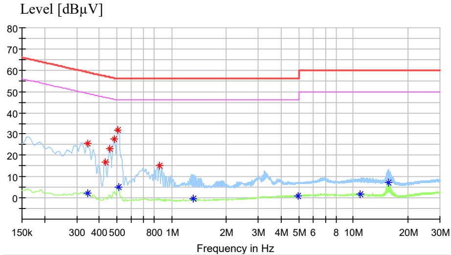
Figure 4: Spectral Diagrams, Conducted Emission, 150 kHz – 30 MHz, mode 2, N line
