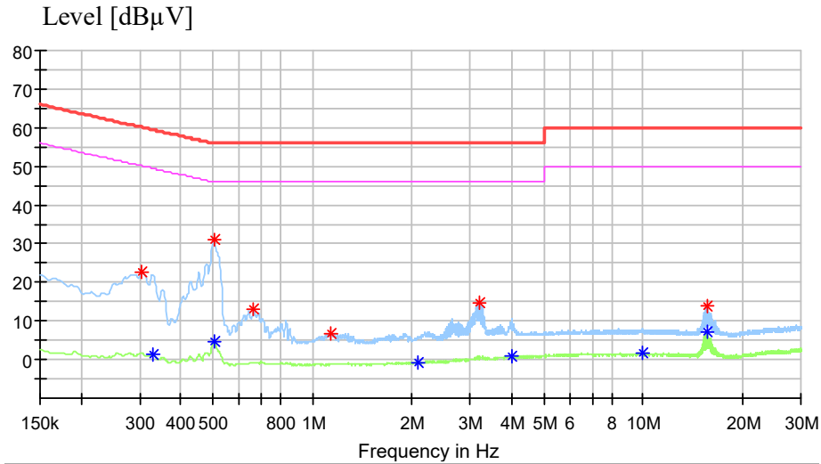
Figure 3: Spectral Diagrams, Conducted Emission, 150 kHz – 30 MHz, mode 2, L line
