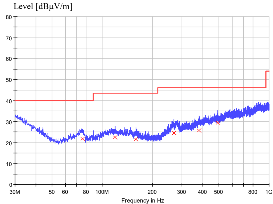
Figure 5: Spectral diagrams, radiated emission, 30 MHz – 1000 MHz, mode 1, horizontal polarization
