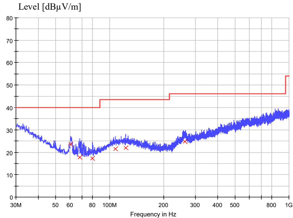
Figure 8: Spectral diagrams, radiated emission, 30 MHz – 1000 MHz, mode 2, vertical polarization
