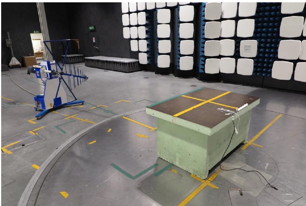
Test set up radiated emission 30 MHz – 1 GHz, with ICPSLC24-10NA-IL-1
