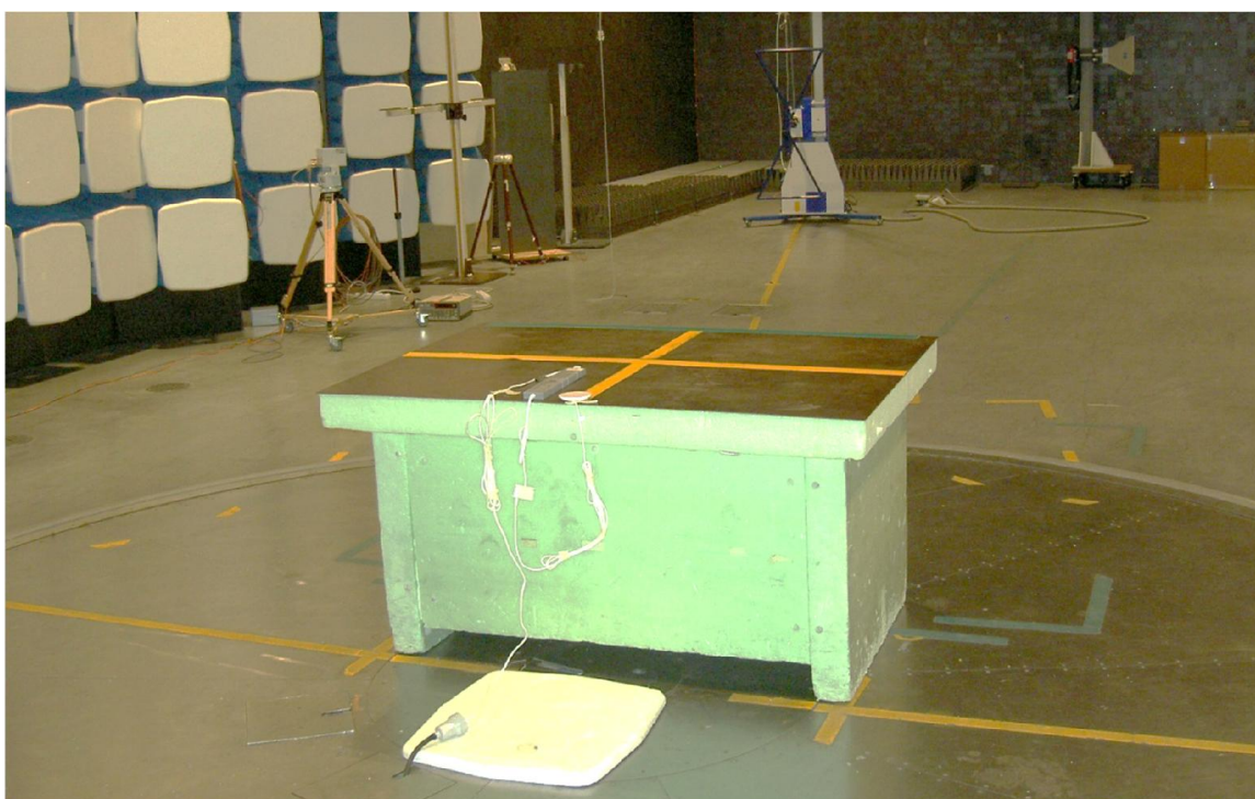
Test set up radiated emission 30 MHz – 1 GHz
