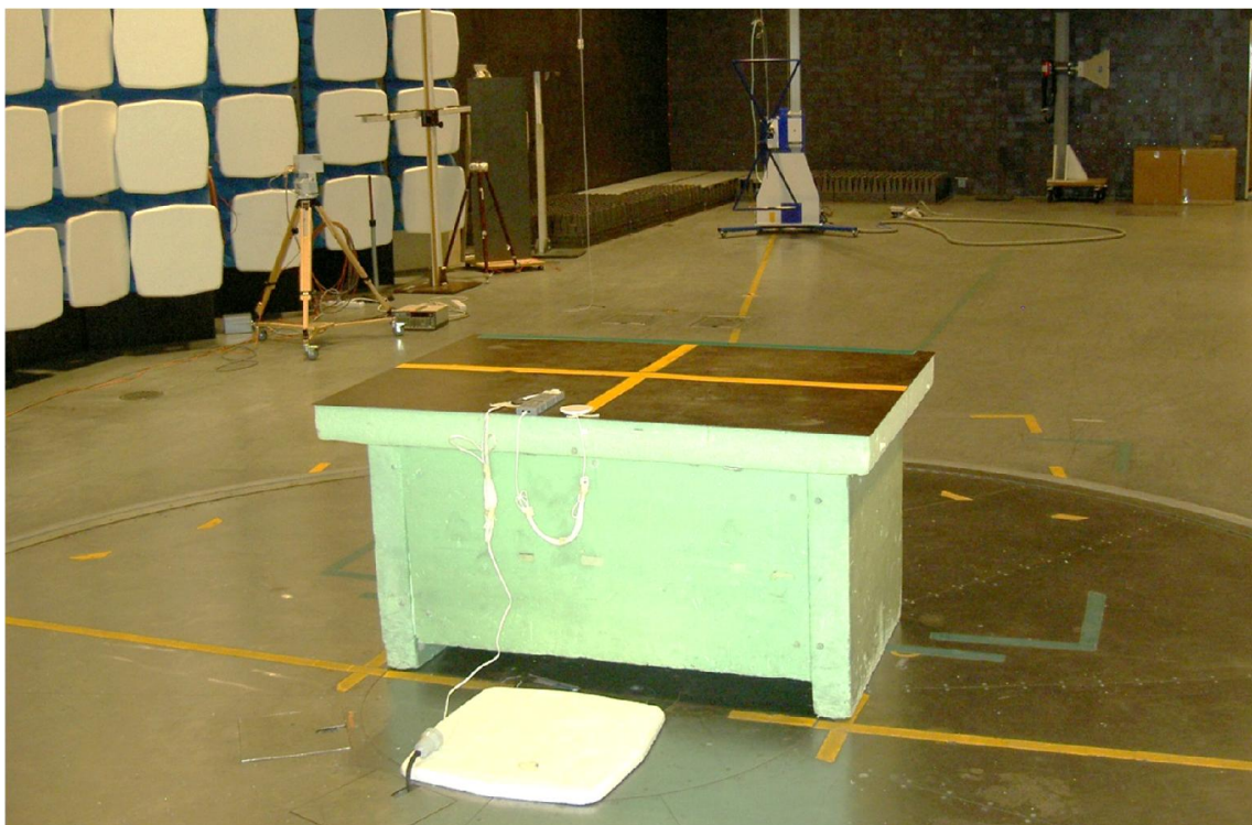
Test set up radiated emission 30 MHz – 1 GHz
