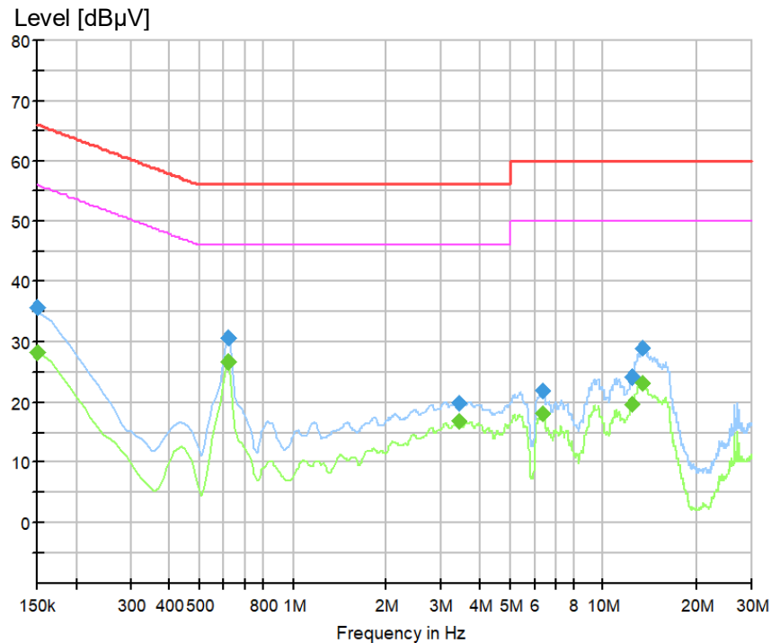
Figure 1: Spectral Diagrams, Conducted Emission, 150 kHz – 30 MHz, L
