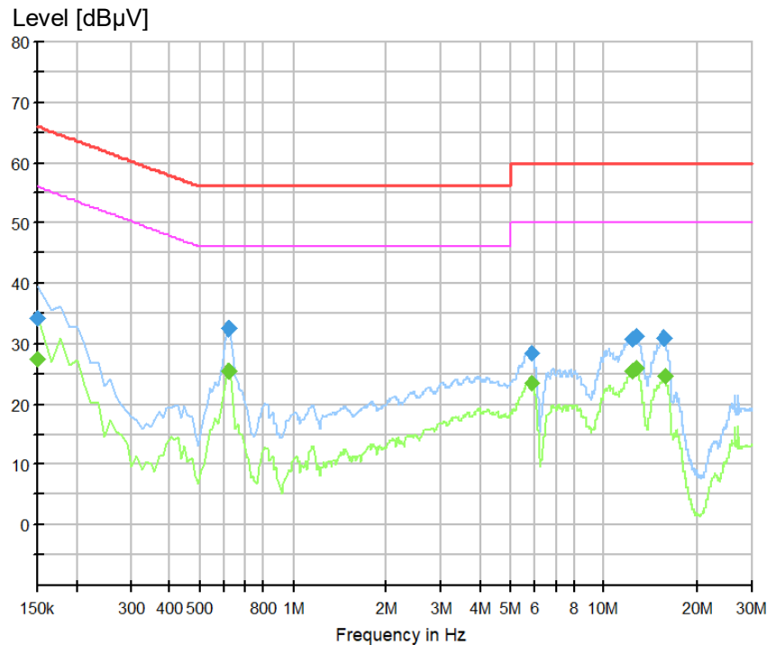
Figure 1: Spectral Diagrams, Conducted Emission, 150 kHz – 30 MHz, L
