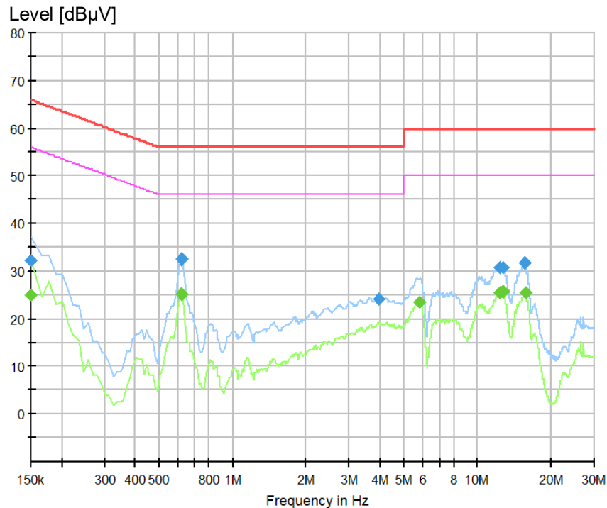
Figure 2: Spectral Diagrams, Conducted Emission, 150 kHz – 30 MHz, N
