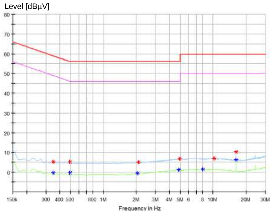
Figure 1: Spectral Diagrams, Conducted Emission, 150 kHz – 30 MHz, L with power supply
