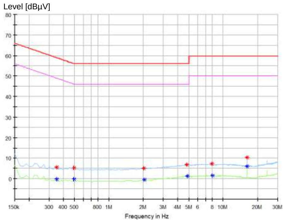
Figure 2: Spectral Diagrams, Conducted Emission, 150 kHz – 30 MHz, N with power supply
