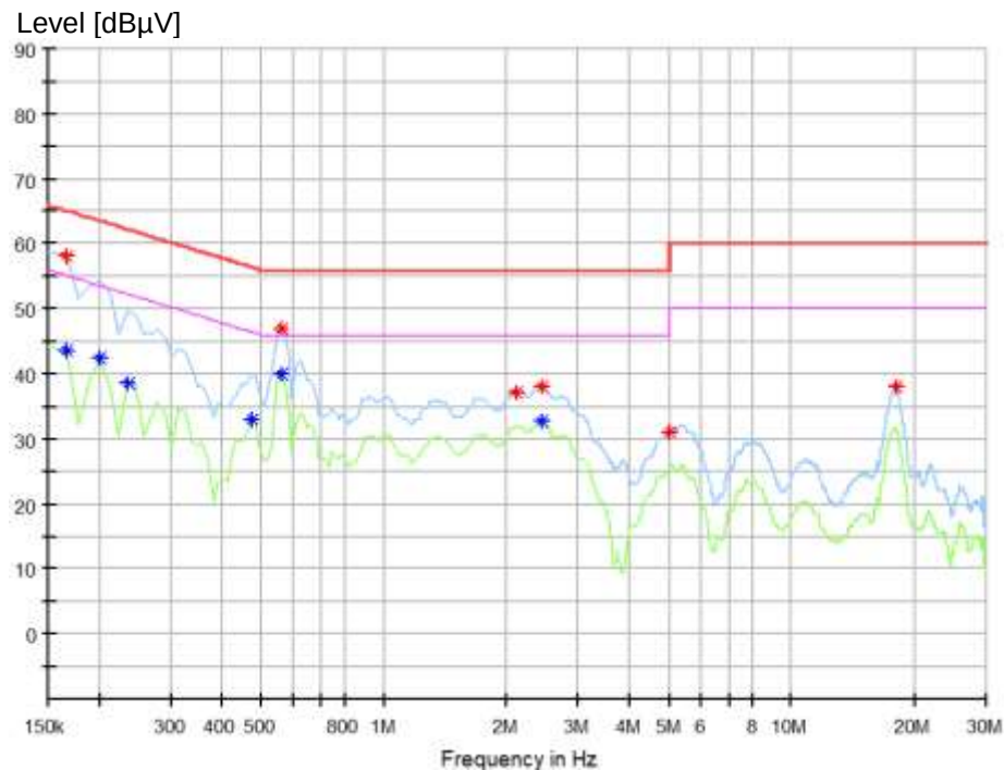
Figure 3: Spectral Diagrams, Conducted Emission, 150 kHz – 30 MHz, L with computer
