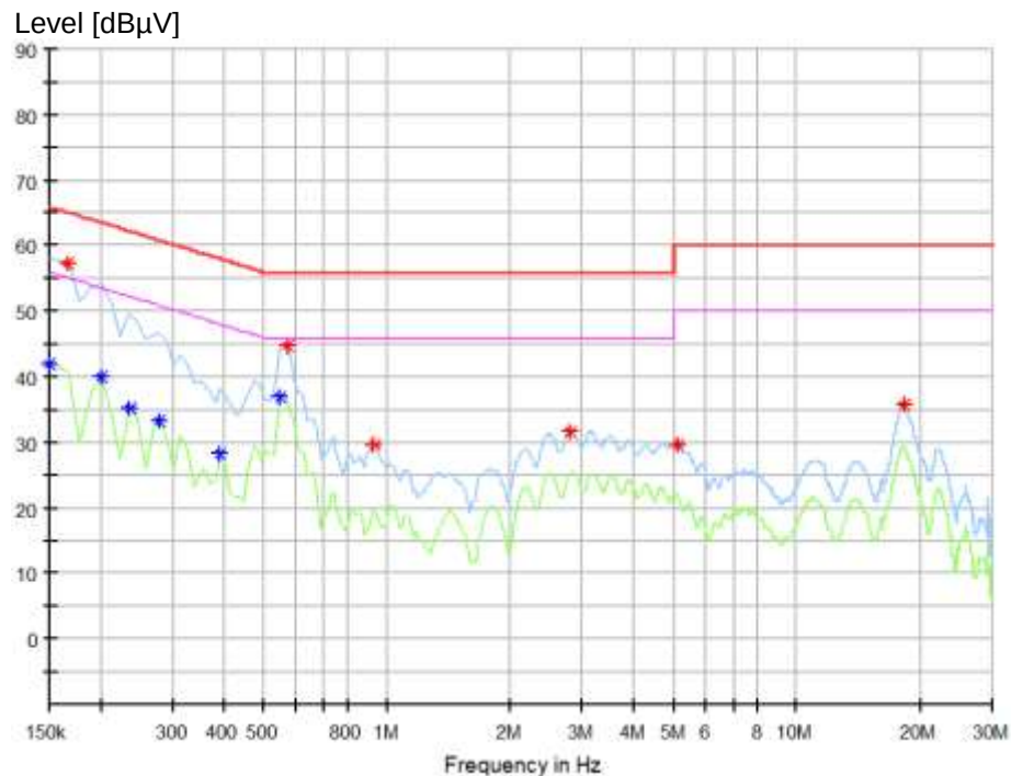
Figure 4: Spectral Diagrams, Conducted Emission, 150 kHz – 30 MHz, N with computer
