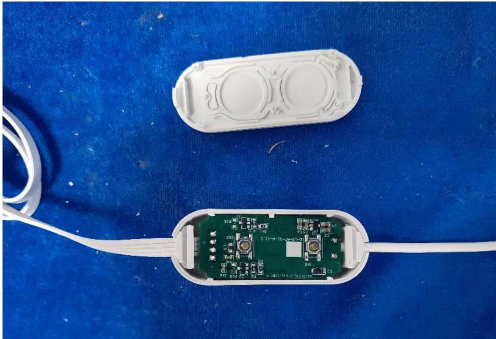
Inside view of switch control box
