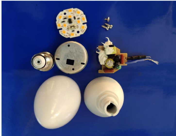
Exploded view
