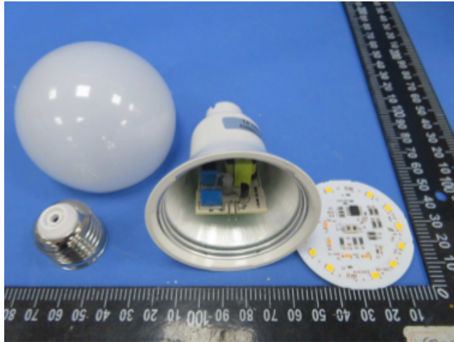
Exploded view
