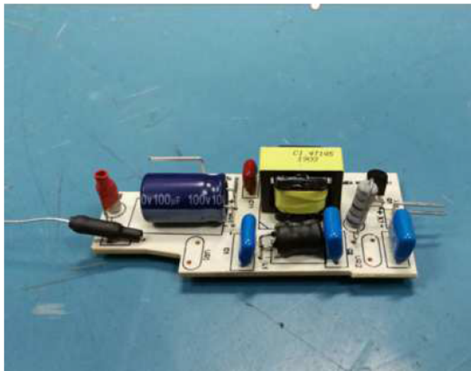
PCB top view
