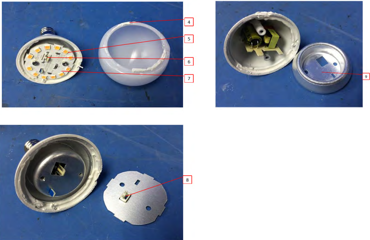
Exploded View
