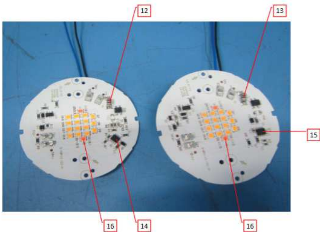
Photo 7 - Alternative driver PCB (Left - U1: BP5178FLD; Right - U1: SY59108N)
