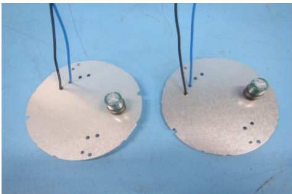
Photo 8 - Alternative driver PCB (Left - U1: BP5178FLD; Right - U1: SY59108N)
