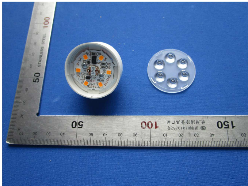
Inside overview
