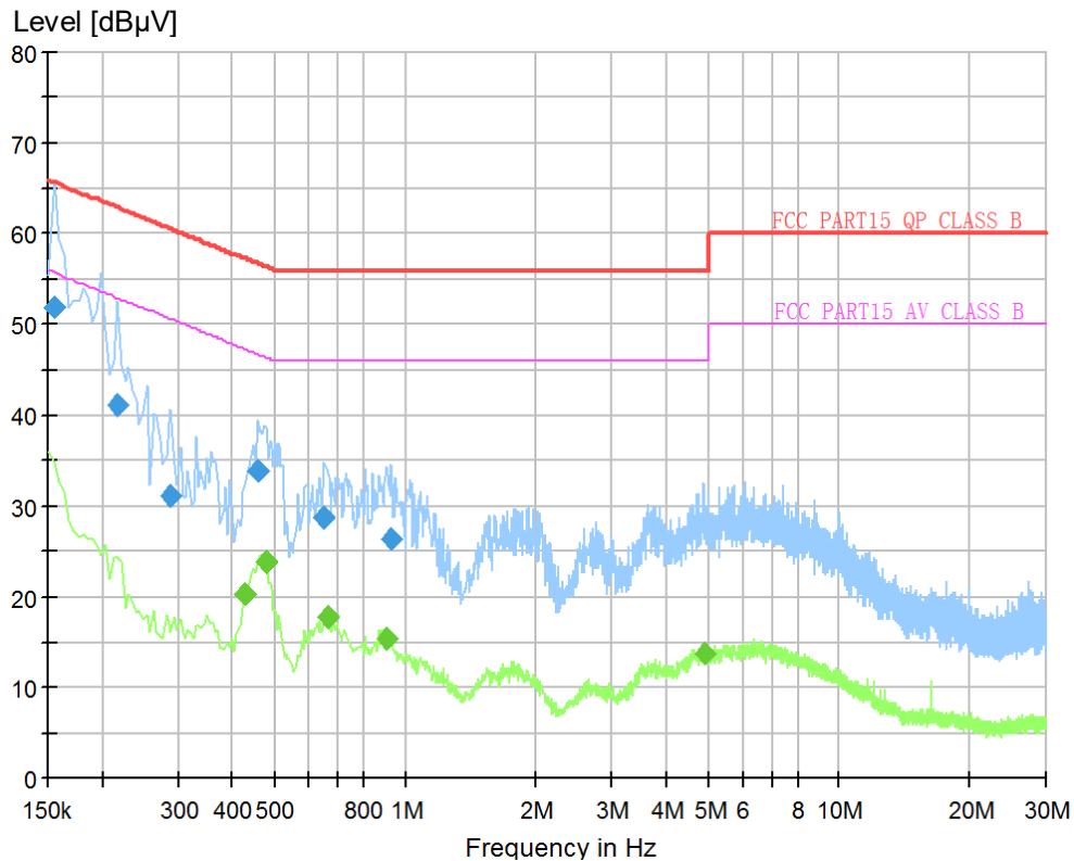
Figure 2: Spectral diagram and measurement results, conducted emission, 150 kHz – 30 MHz, line N
