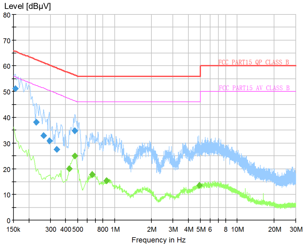
Figure 1: Spectral diagram and measurement results, conducted emission, 150 kHz – 30 MHz, line L
