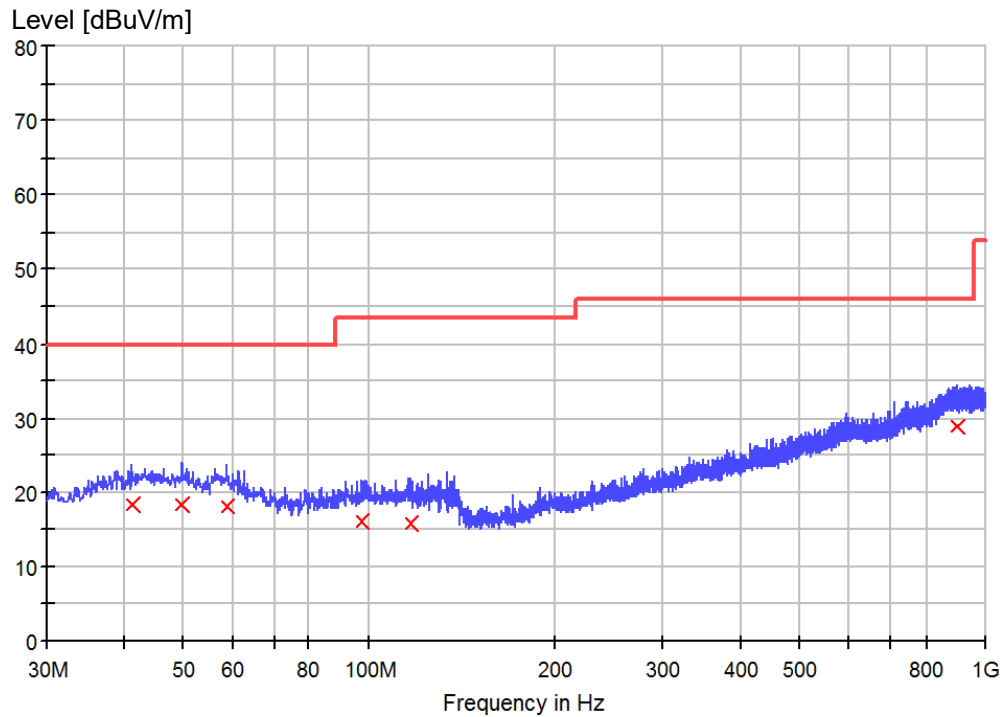
Figure 3: Spectrum diagrams and measurement results, radiated emission, 30-1000 MHz, Horizontal polarization
