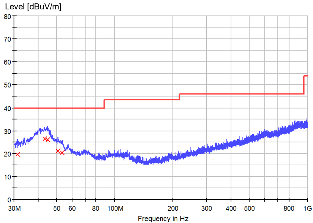
Figure 4: Spectrum diagrams and measurement results, radiated emission, 30-1000 MHz, Vertical polarization
