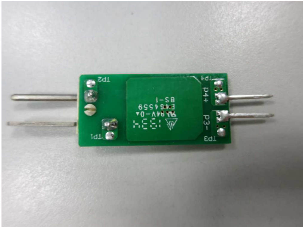
Rear of PCB
