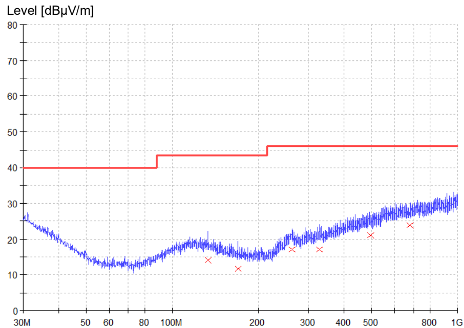
Figure 1: Spectral Diagrams, Radiated Emission, 30 MHz – 1000 MHz, Horizontal polarization, DC 24 V
