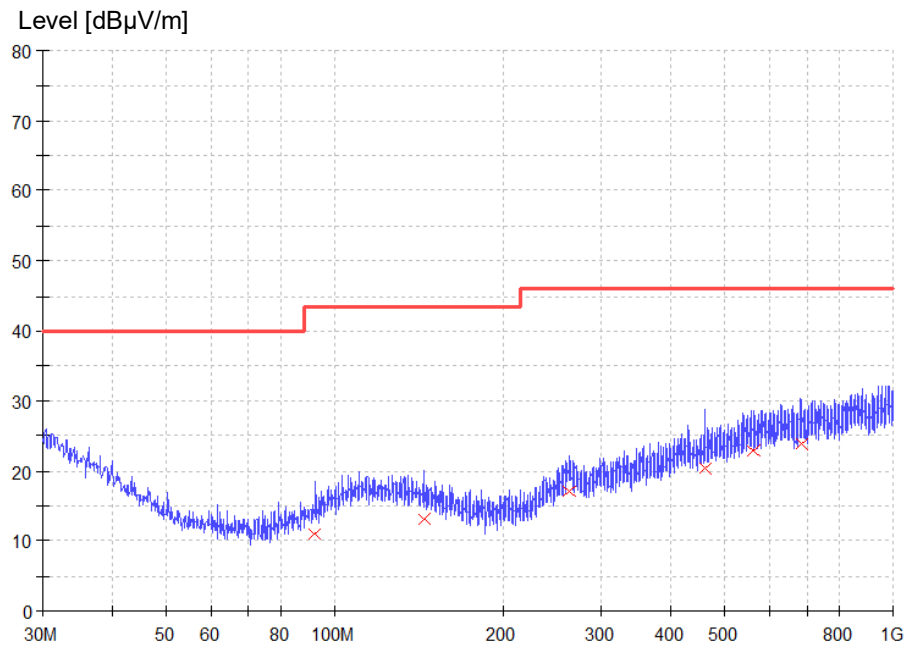
Figure 2: Spectral Diagrams, Radiated Emission, 30 MHz – 1000 MHz, Vertical polarization, DC 24 V
