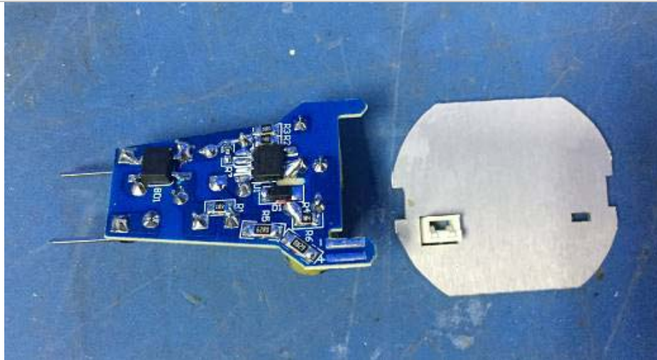
PCB view
