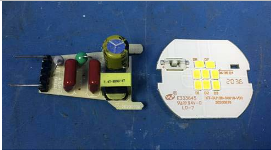
PCB view
