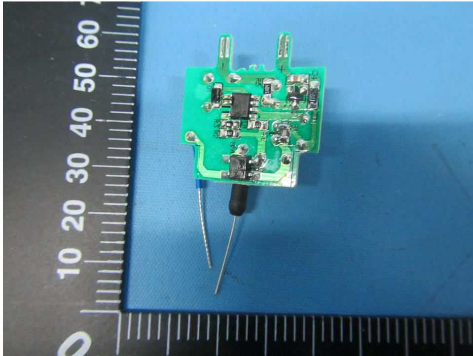
Photo 4 - Internal view
