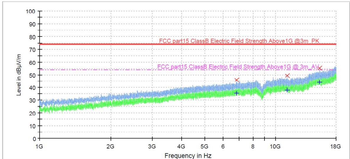
Figure 5: Spectral Diagrams, Radiated Emission, 1GHz-18GHz, Horizontal polarization
