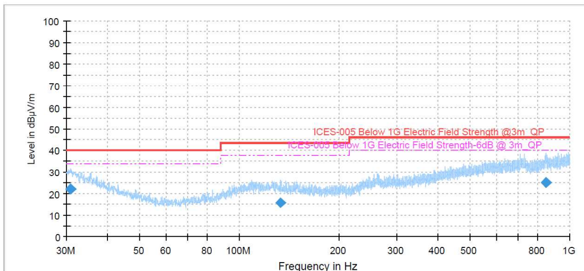
Figure 3: Spectral Diagrams, Radiated Emission, 30MHz-1000MHz, Horizontal polarization
