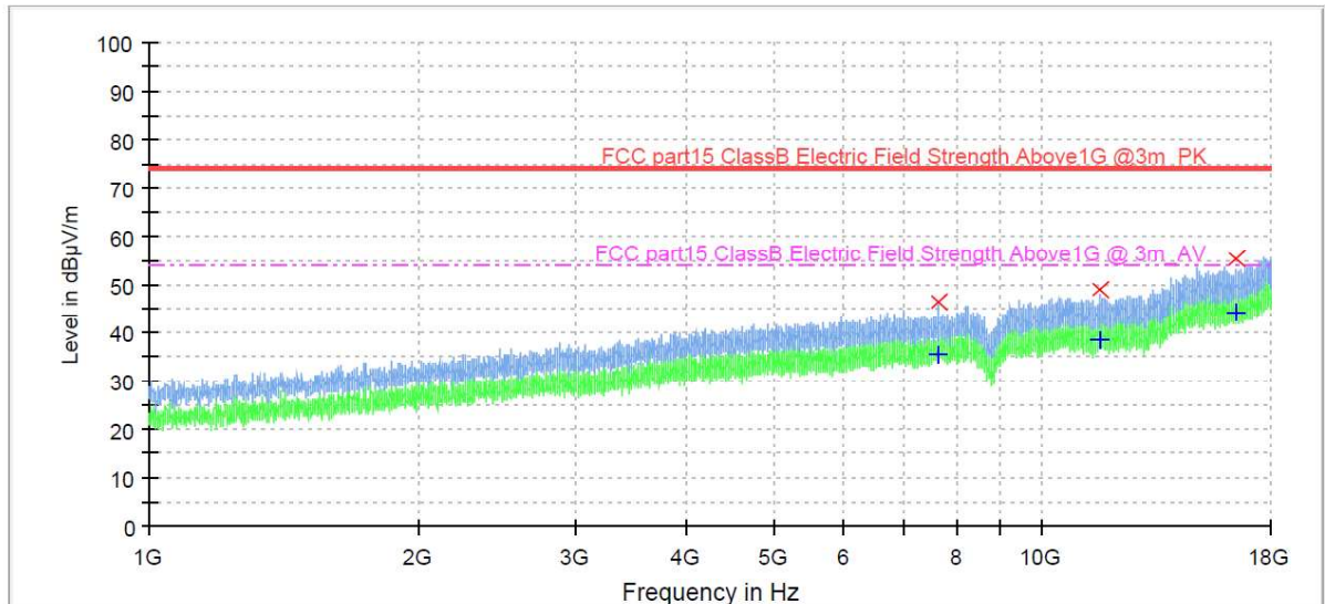
Figure 6: Spectral Diagrams, Radiated Emission, 1GHz-18GHz, Vertical polarization
