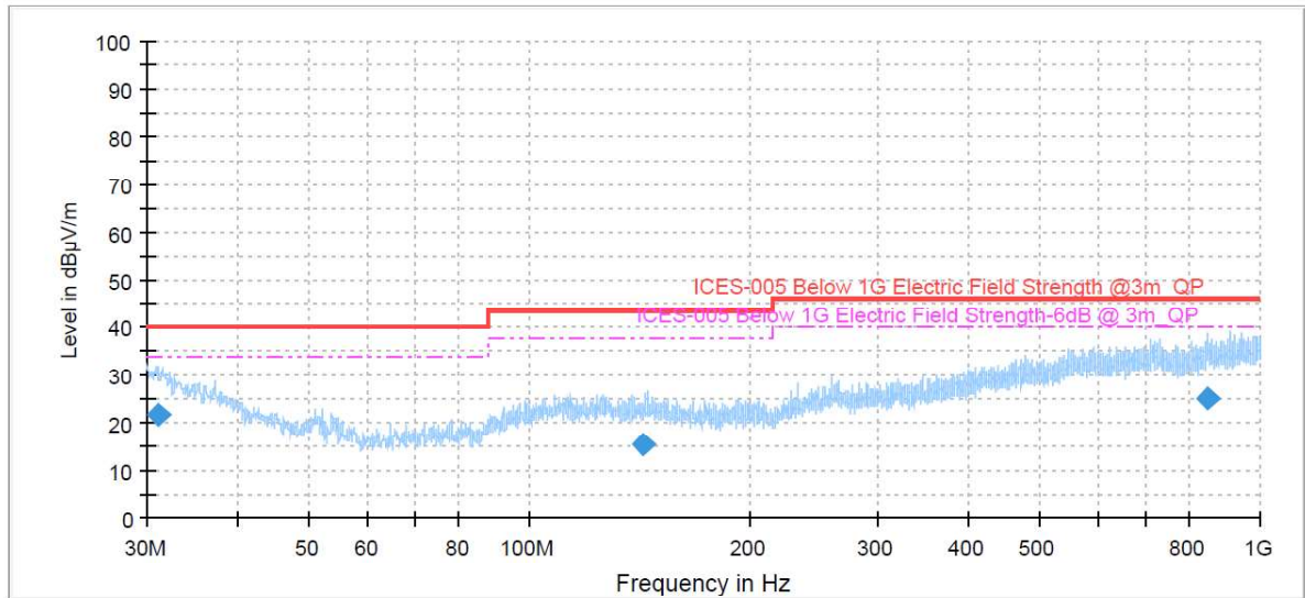
Figure 4: Spectral Diagrams, Radiated Emission, 30MHz-1000MHz, Vertical polarization
