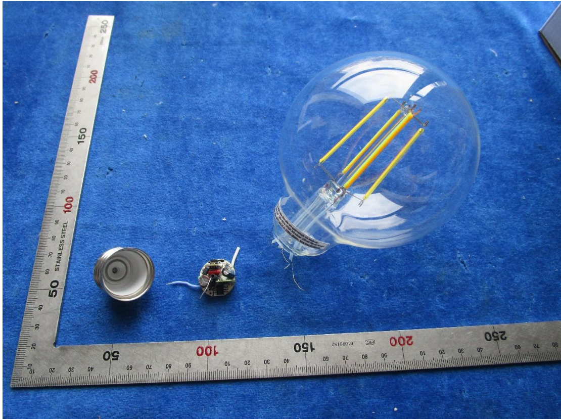
Internal View (with SILABS RF IC)
