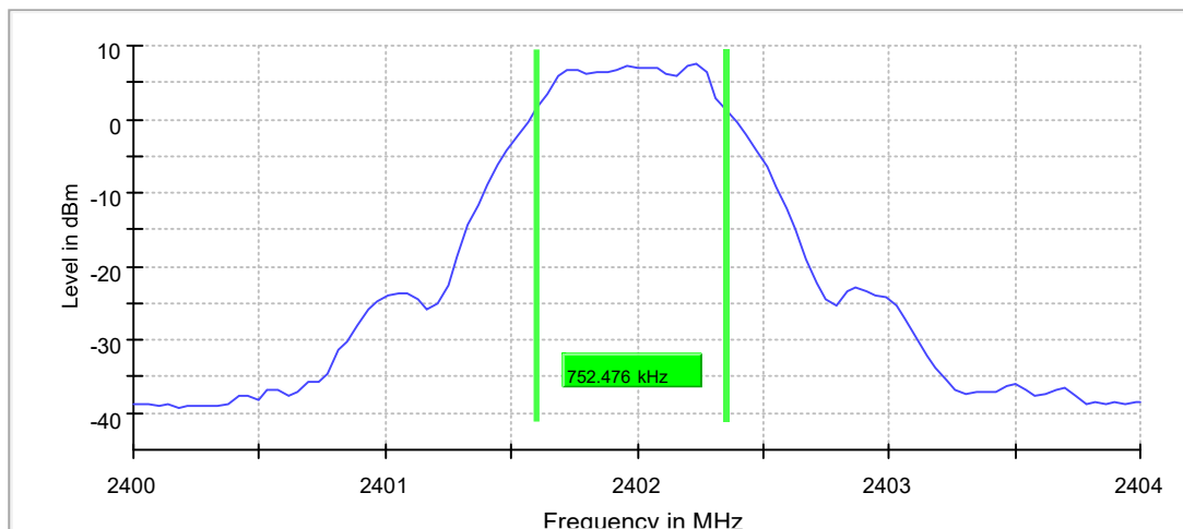
6 dB Bandwidth
