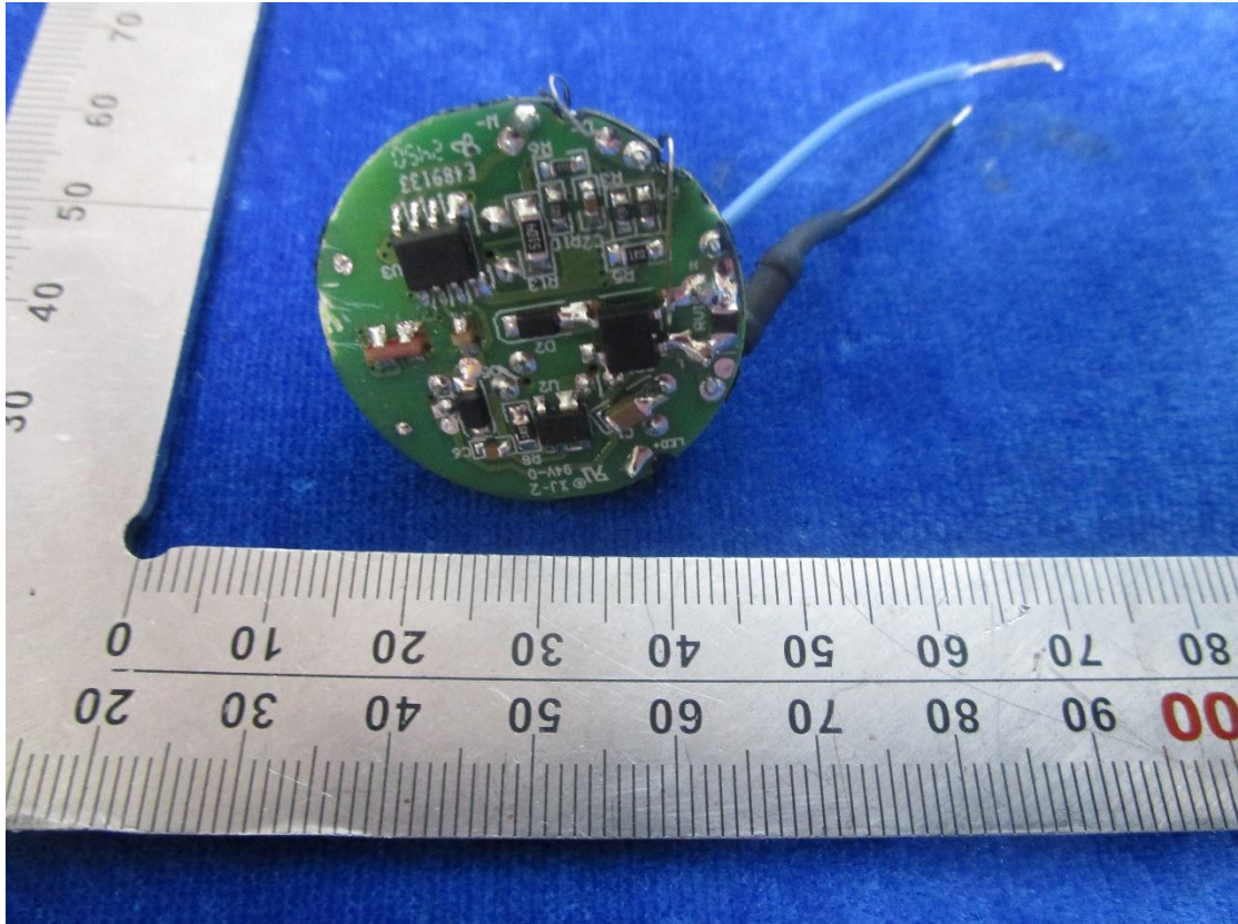
PCB (with SILABS RF IC)
