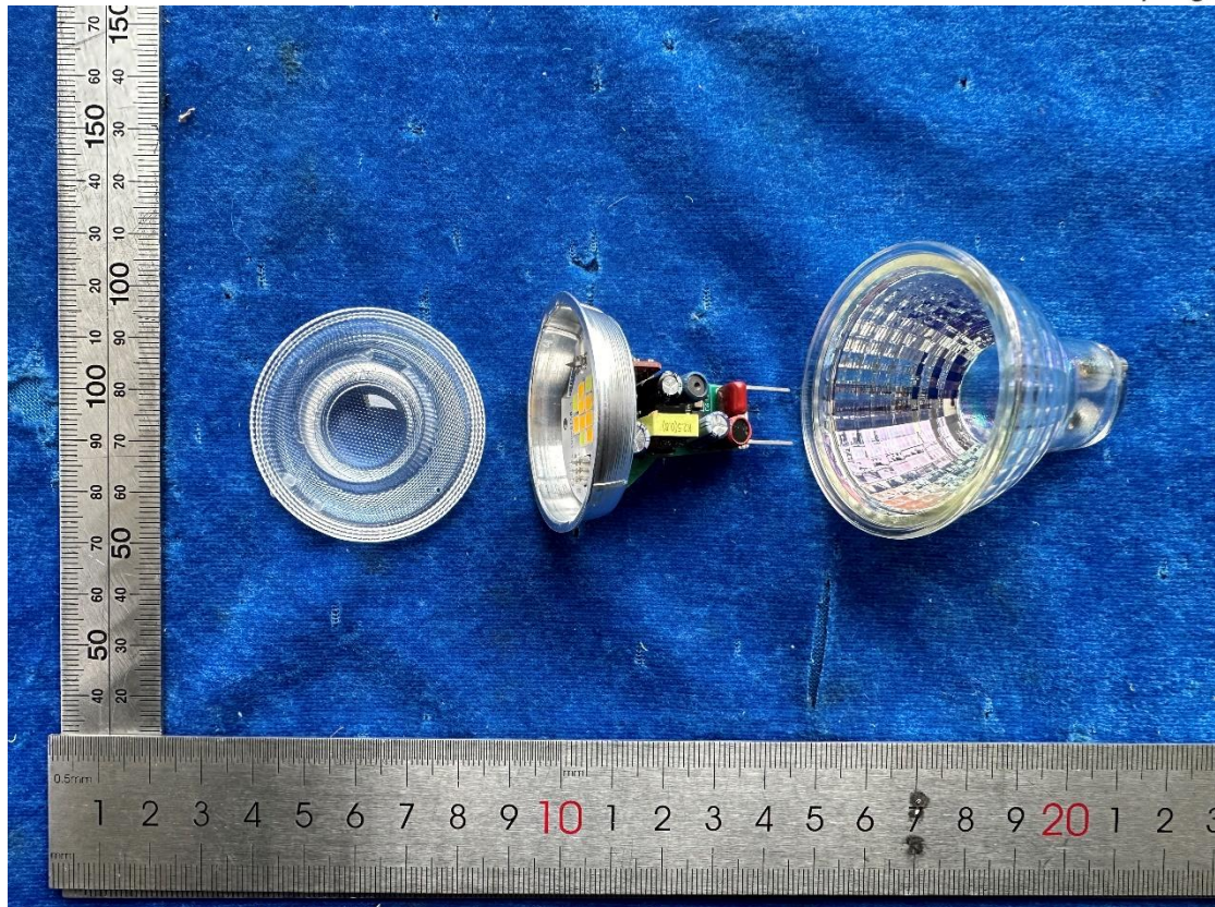
Open View
