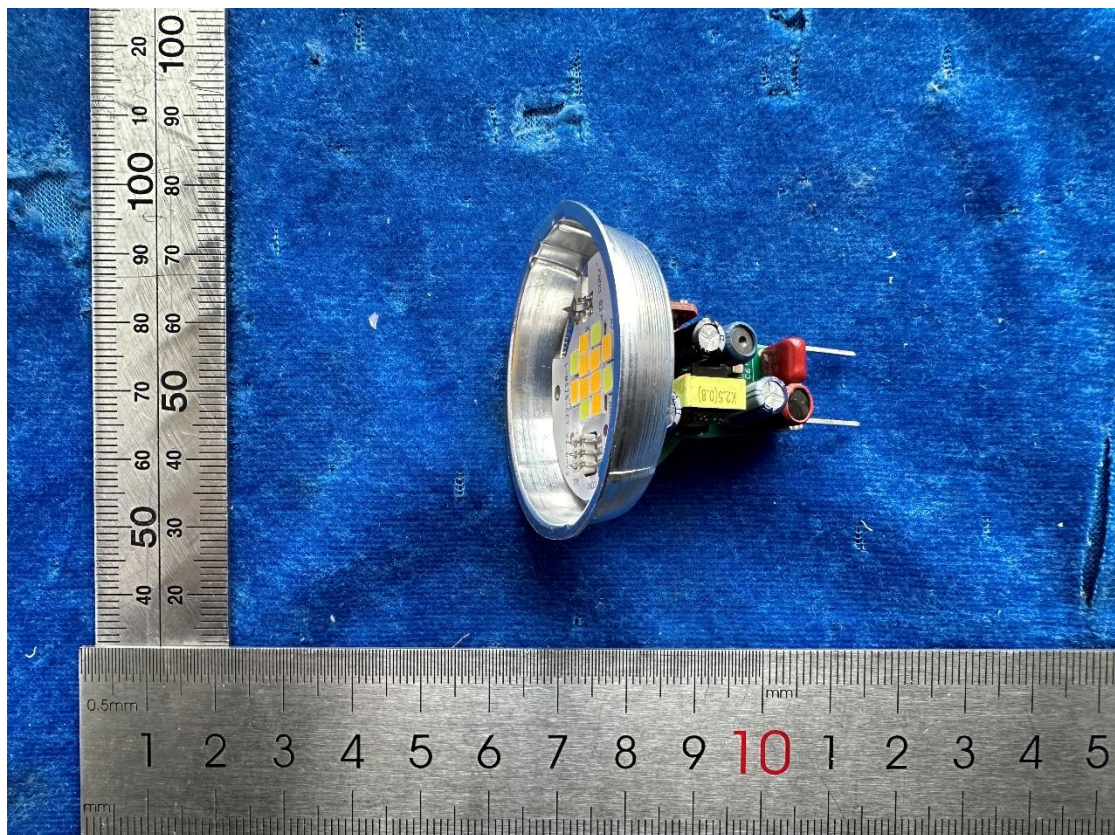
Open View
