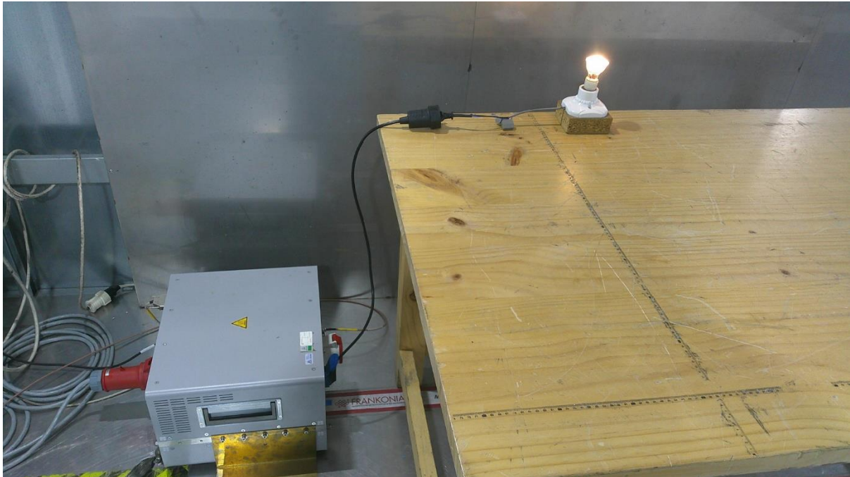
Photograph 2: Set-up for measurement of radiated emission
