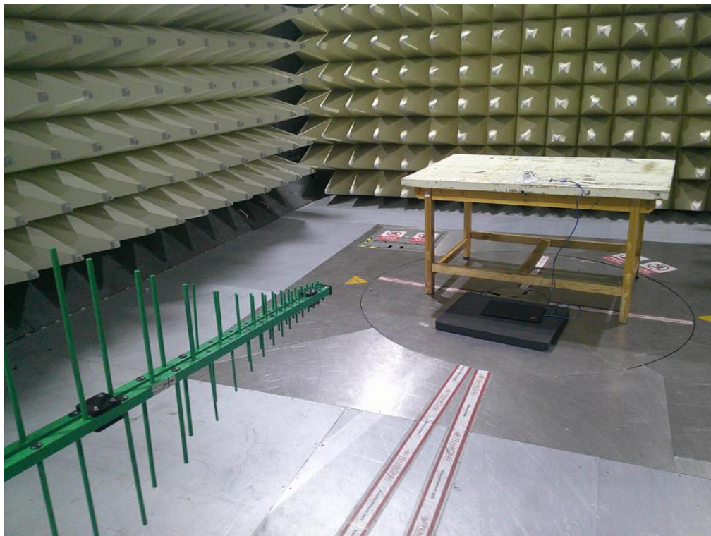
Photograph 3: Set-up photo for Radiated Emission, 30MHz - 1GHz
