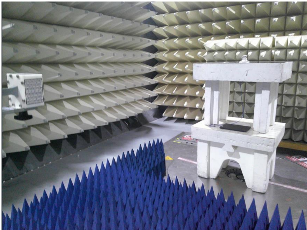
Photograph 5: Set-up photo for Radiated Emission, 18GHz - 25GHz
