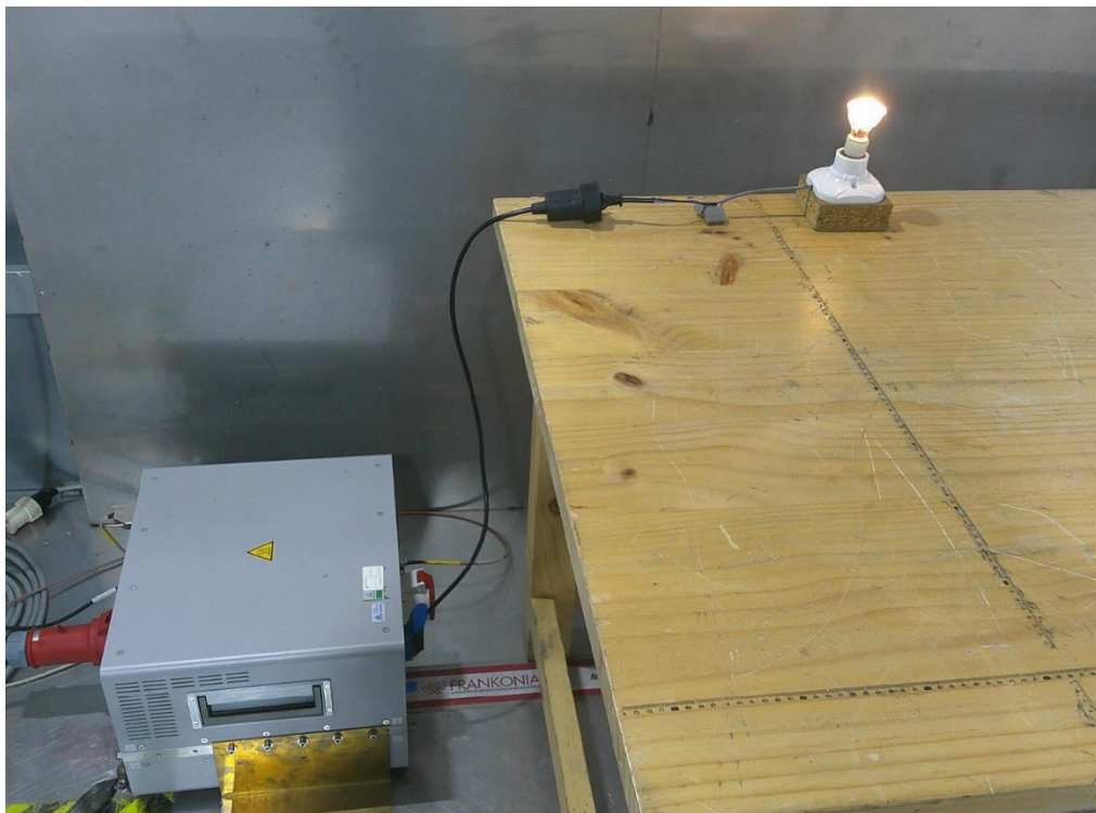
Photograph 2: Set-up photo for Conducted Emission
