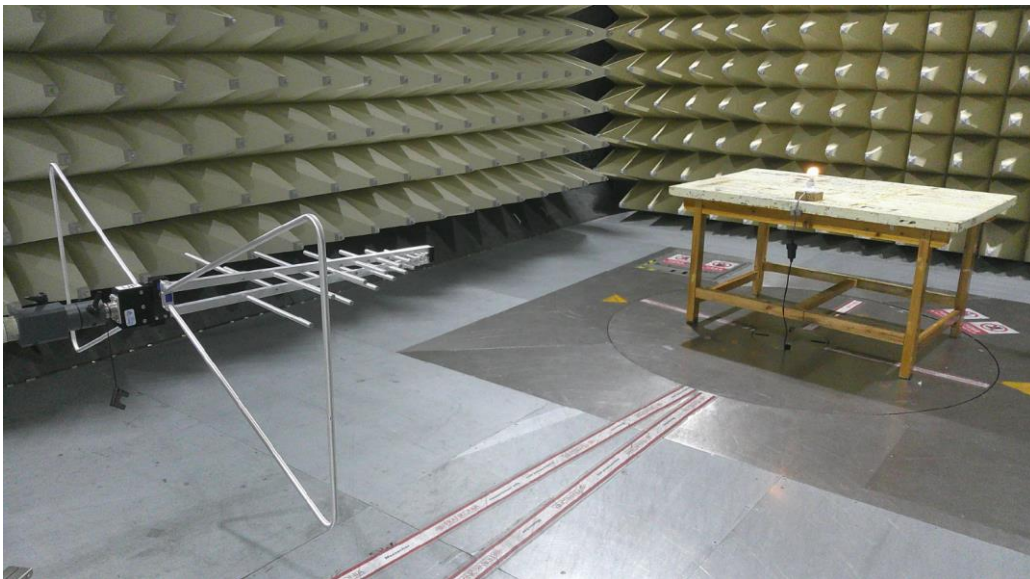
Photograph 2: Set-up for measurement of radiated emission
